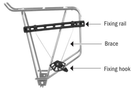
QL3/QL3.1 mounting elements
